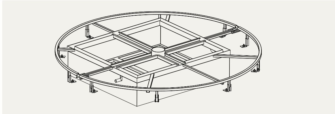
Floor element with drive box for floor pit, measure X = 350 or larger
